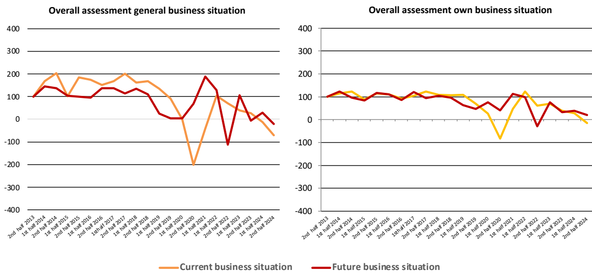
Figure 1: Composites-Development-Index
